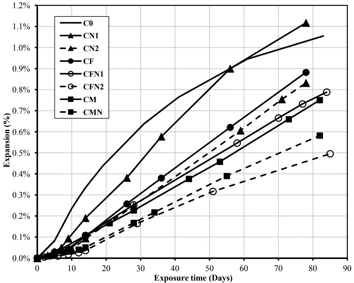
Figure 59 Expansion in mortar bars at different exposure ages.
