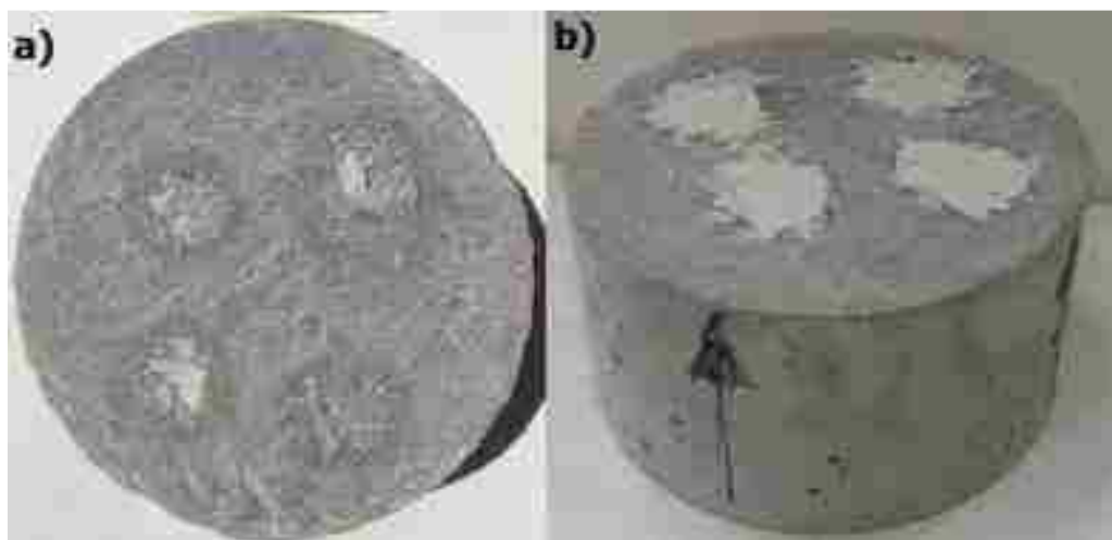
Figure 13 Abrasion specimen A-2 a) after abrasion, b) with clay-filled cavities.
